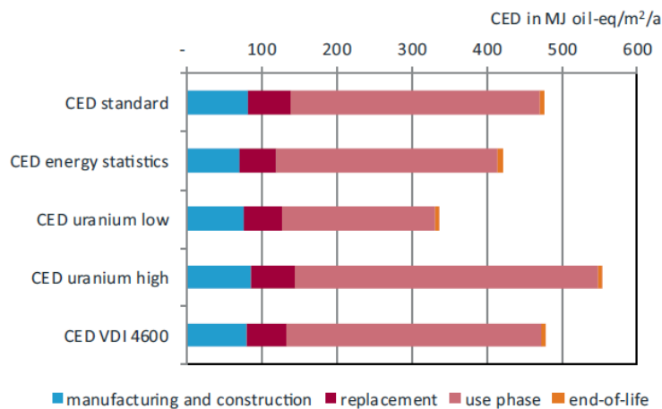
Figure 1-12: Cumulative energy demand of the life cycle of the building Rautistrasse in Zürich, differentiating between manufacturing and construction, replacement, use and end of life of the building (Frischknecht et al. 2015).
