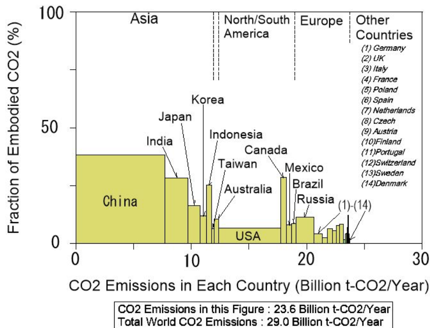
Figure 1-4: Total CO 2 emissions in each country and the fraction of embodied CO 2 (Oka et al., 2014).
