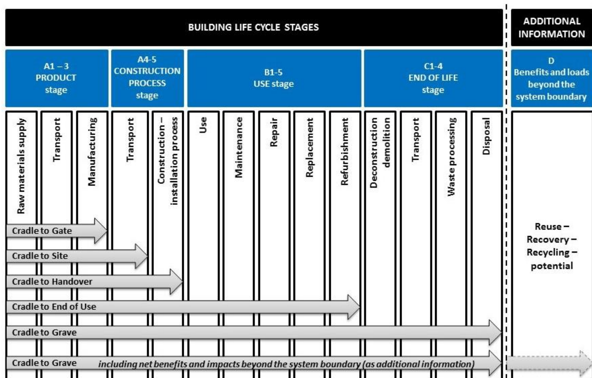
Figure 1-11: Overview of the various existing system boundary types using the respective modules of building life cycle model developed by the group CEN TC 350 (EN 15978:2011). (Balouktsi & Lützkendorf, 2016)
