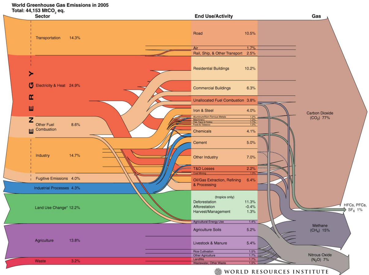
Figure 1-3: World Greenhouse Gas Emissions in 2005 per sector according to WRI (Herzog, 2005).
