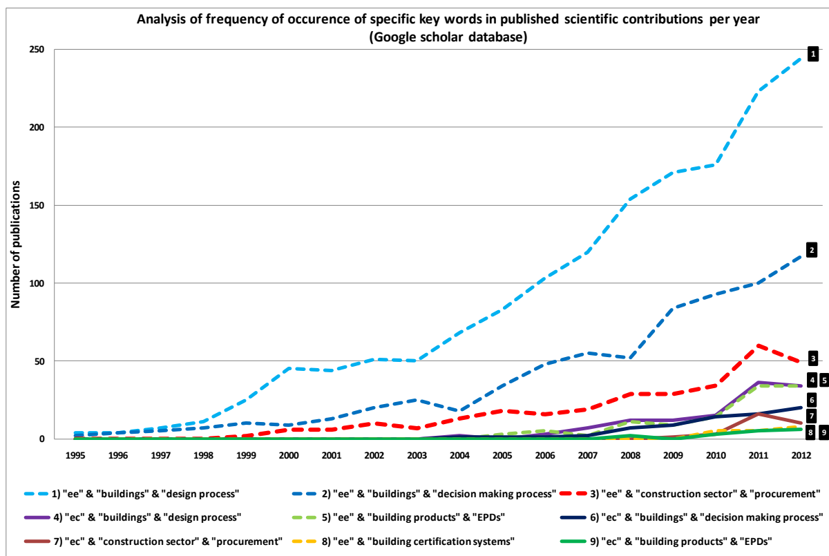
Figure 1-7: Investigation of the trends in research using the key words “design process”, “procurement”, “decision making process”, “building certification systems” and “EPDs” together with “buildings” or “construction sector” and “embodied energy” (dashed lines) or “embodied carbon”.
