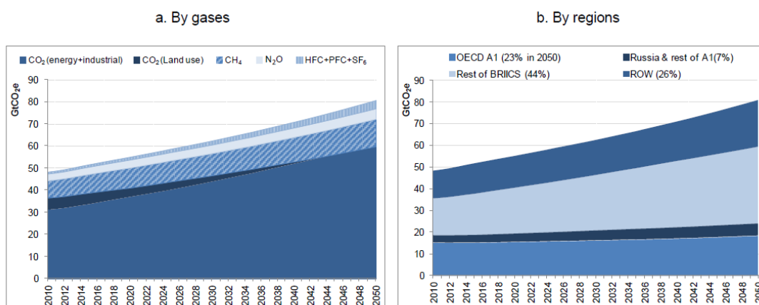
Figure 1-2: GHG emissions by region according to the Organisation for Economic Co-operation and Development (OECD): baseline scenario 2010-2050 (Marchal et al., 2011). 6
