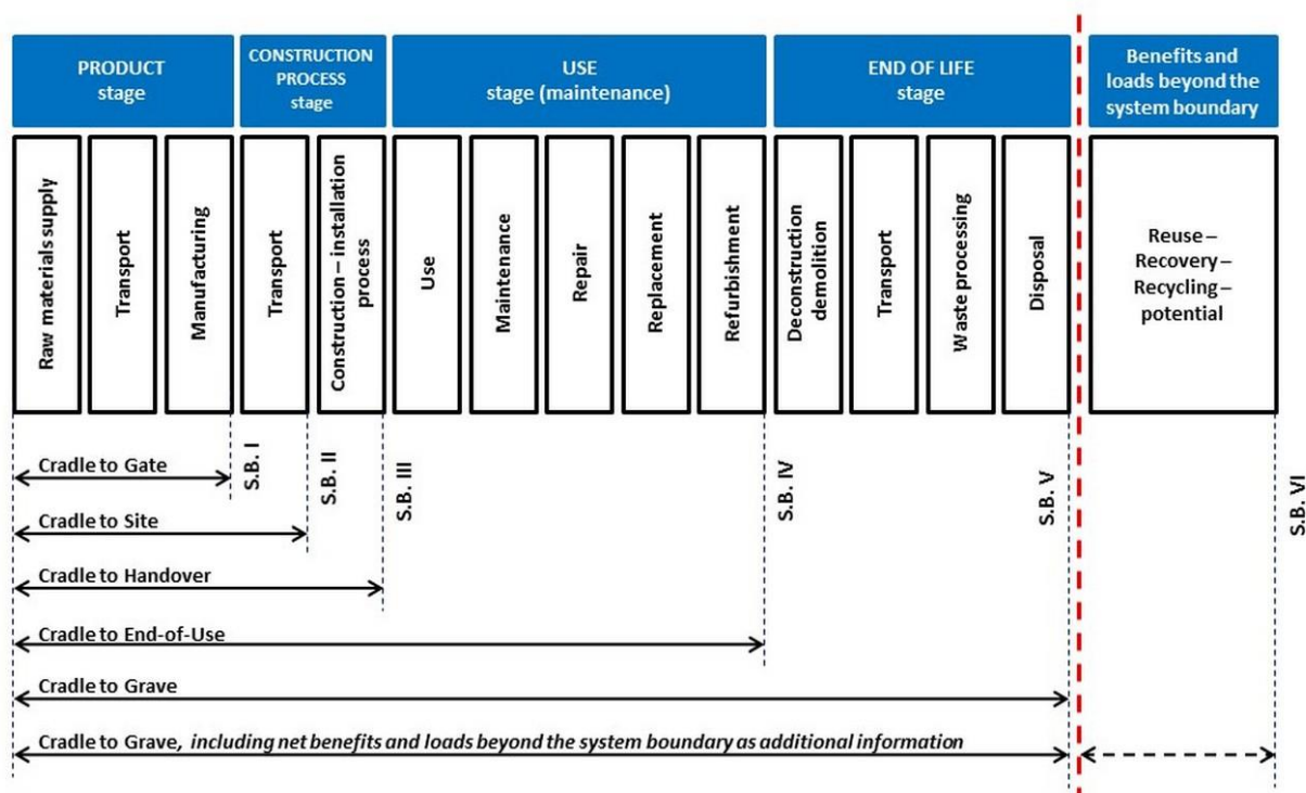
Figure 2-1: Proposed model for system boundary description and selection
