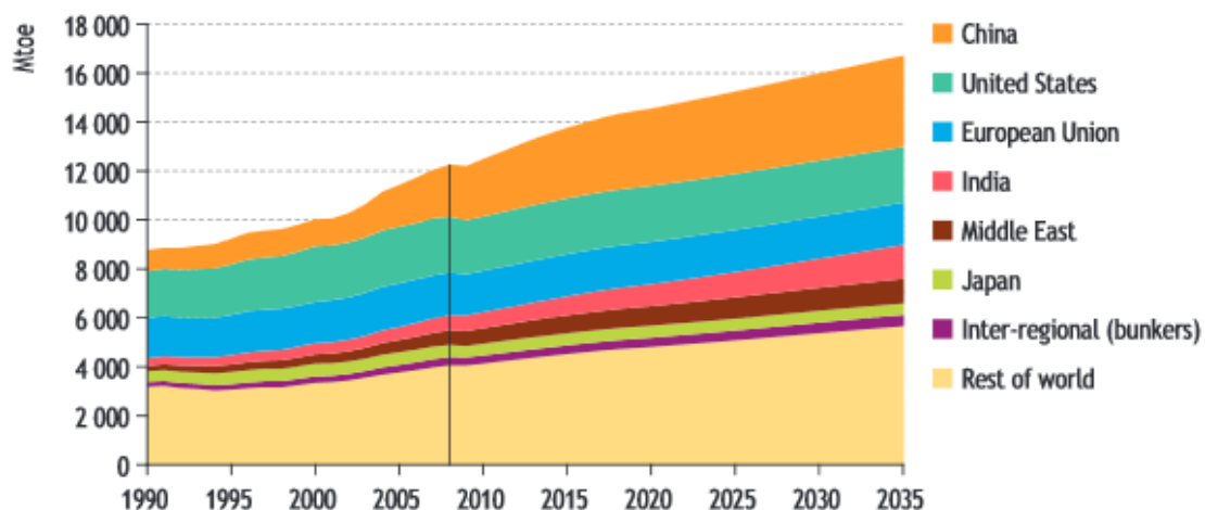
Figure 1-1: Projected growth in primary energy demand between 2010–2035 worldwide (New Policies Scenario). (IEA, 2011)
