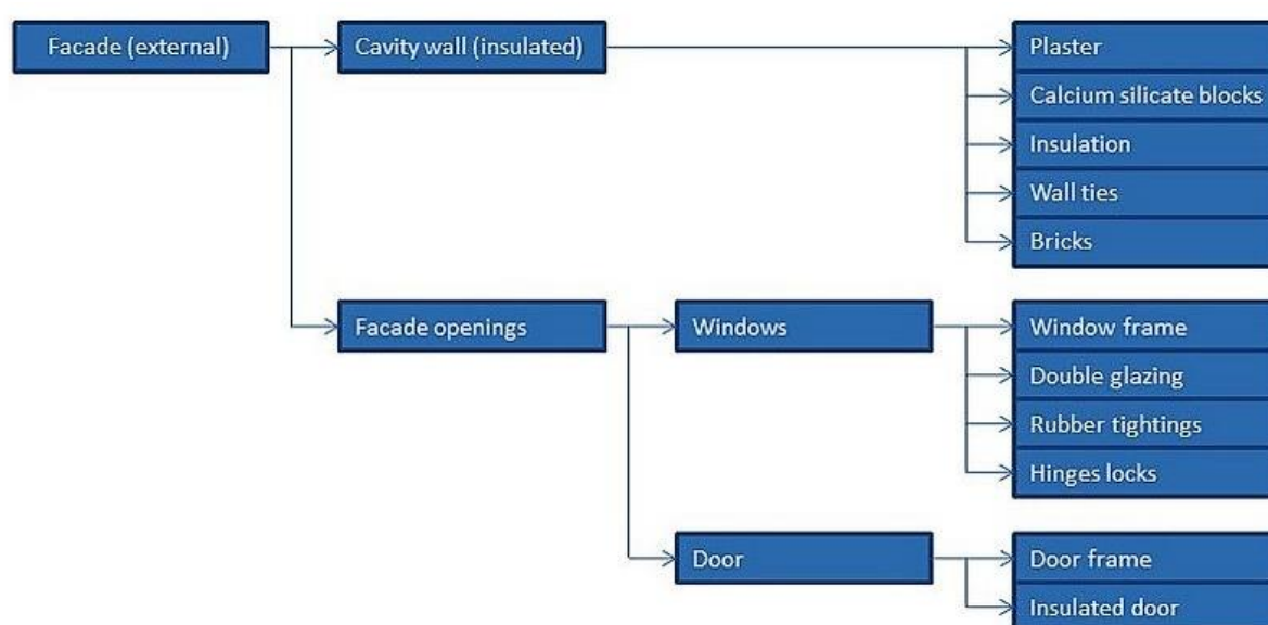
Figure 1-8: Example of a structuring of building information using the different level of aggregation specifically for foundation, frame wall and facade (EN 15978:2011).
