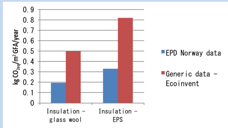
Figure 5.4 Comparison of the use of generic data vs. product specific national data (Source: Subtask 4 report)
