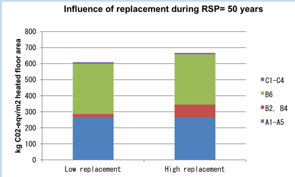
Figure 5.3 Influence of replacement (Source: Subtask 4 report)
