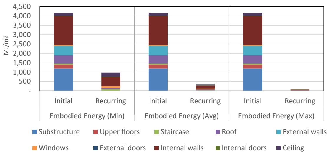
Figure 4.10 Embodied energy of residential building (50 years life span) (Source: Subtask 3 report)
