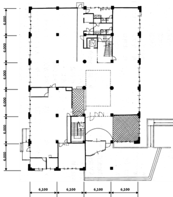
(a) Ground floor layout (BCI, 2004)
