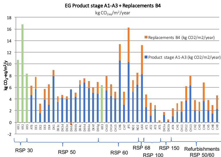
Figure 5.6 Cradle-to-gate + replacement EG from Annex 57 case studies (Source: Subtask 4 report)
