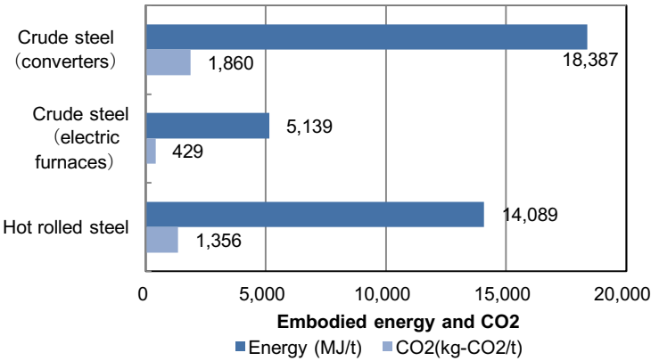
Figure 4.9 Embodied energy and GHG emissions of Steel (Source: Yokoyama, K., 2015)
