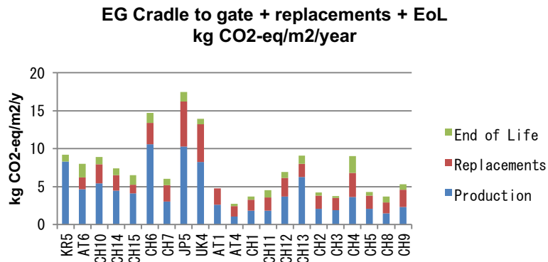
Figure 5.5 Cradle to gate + replacements + EOL EG from available Annex 57 case studies (Source: Subtask 4 report)
