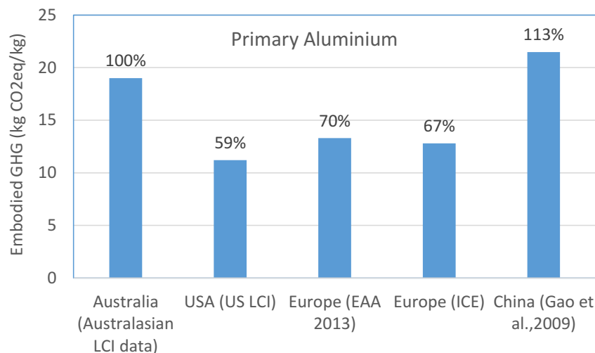
Figure 4.5 Embodied GHG emissions of Aluminium comparison for different countries (Source: Subtask 3 report)
