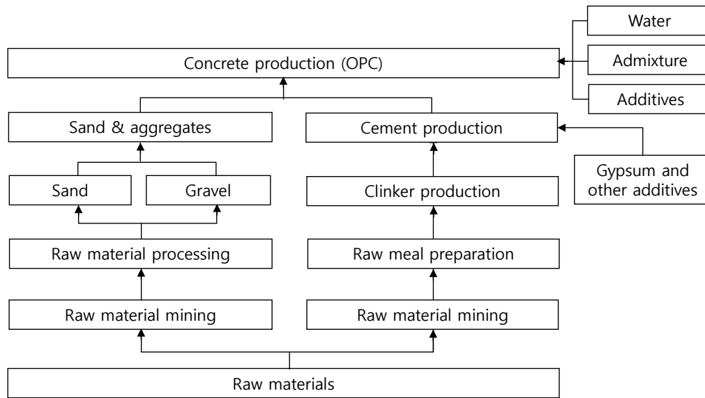
Figure 4.4 Process map for OPC (Source: Subtask 3 report)
