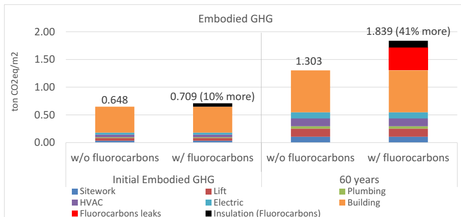
Figure 4.7 Embodied GHG emissions of example building (Source: Subtask 3 report)
