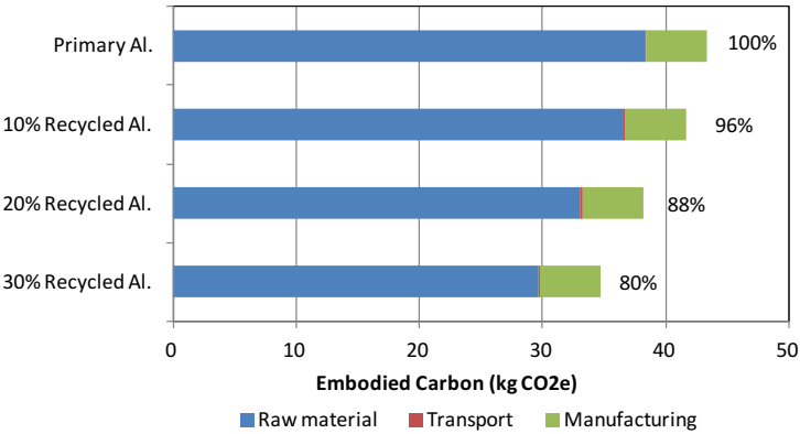
Figure 4.8 Embodied GHG emissions comparison between different recycled aluminium for window (Source: Subtask 3 report)
