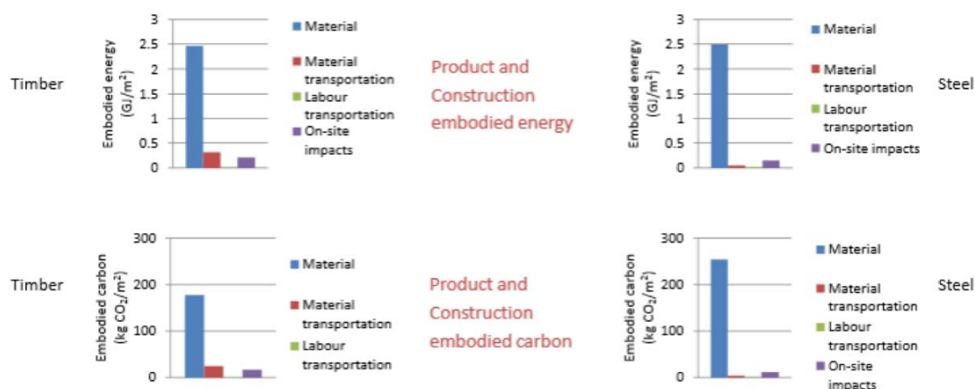
Figure 5.9 Results of the UK case study with the code name UK7 (Source: Subtask 4 report)
