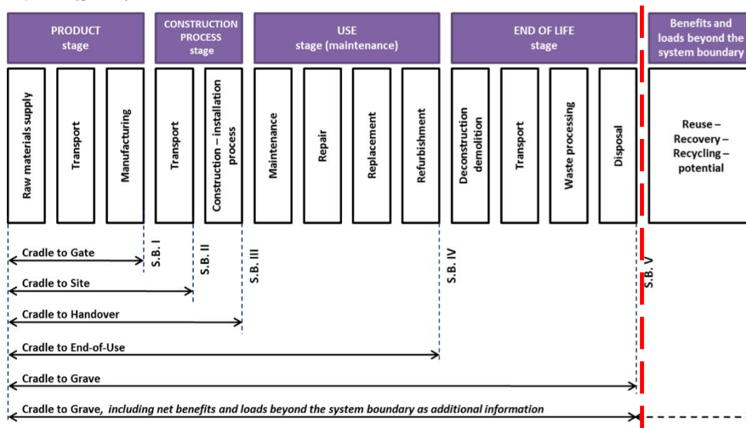
Figure 3.2 Proposed model for system boundary description and selection (Source: Subtask 1 report)
