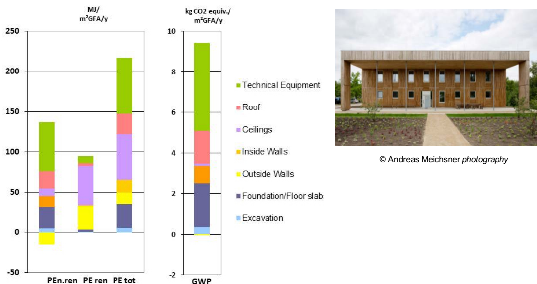
Figure 5.7 Results of the German case study with the code name DE4 (Source: Subtask 4 report)
