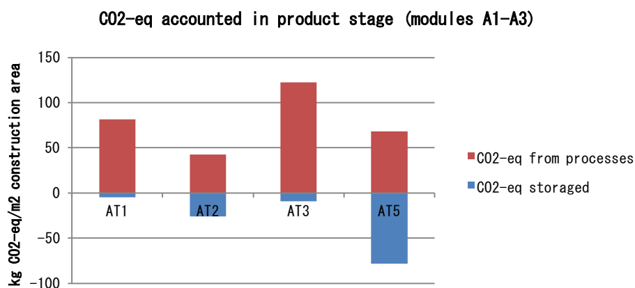
Figure 5.8 Embodied GHG emissions from cradle to gate of Austrian Annex 57 case studies (Source: Subtask 4 report)
