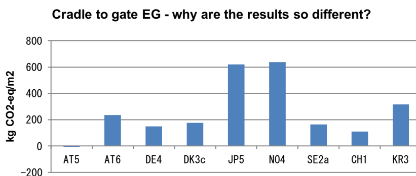
Figure 5.2 Embodied GHG emissions from the cradle to gate stage of different Annex 57 case studies (Source: Subtask 4 report)
